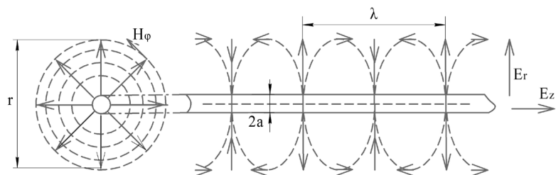
Fig. 5. Structure of the surface wave electromagnetic field E_{00}
