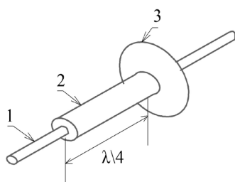
Fig. 7. Fragment of a surface wave wire with a flat reflector: 1 – surface wave wire; 2 – quarter-wave segment; 3 – flat reflector
