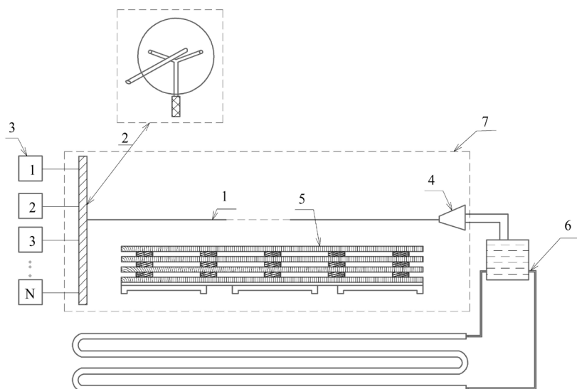
Fig. 9. Large-sized lumber uniform drying system based on MW radiation
