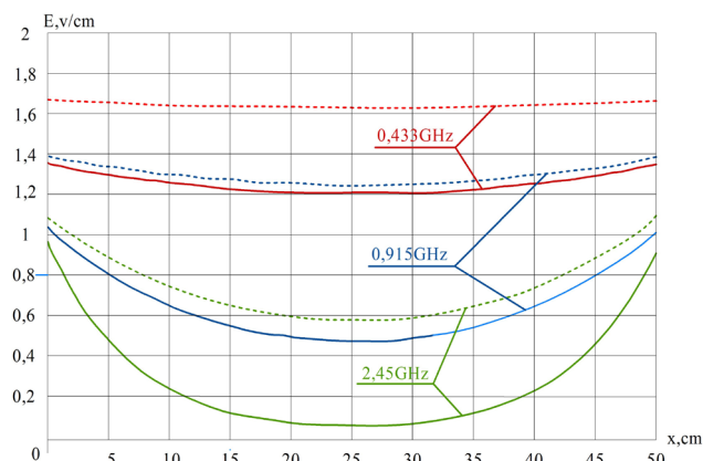
Fig. 2. Graph of the total electric field strength during two-way microwave irradiation of a package of lumber 50 centimeters thick
