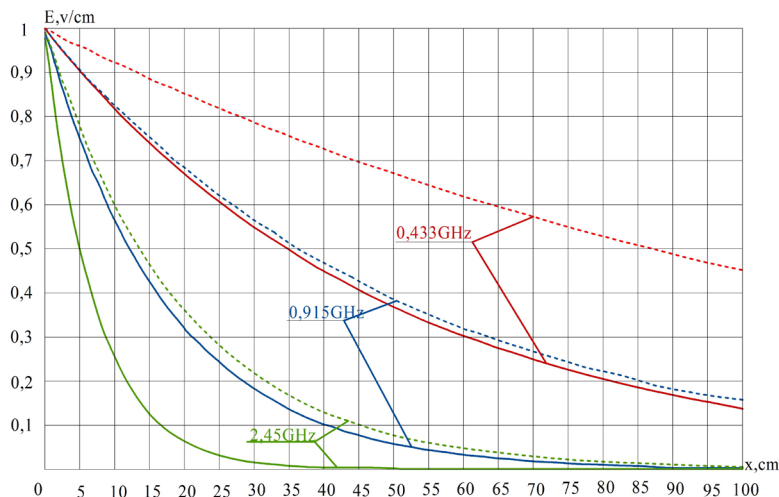
Fig. 1. Graph of the dependence of the electric field strength on the depth of penetration of the microwave field into the wood at different frequencies
