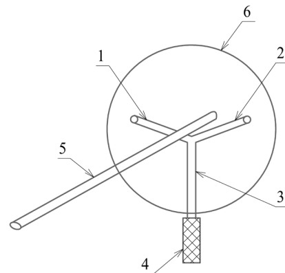
Fig. 6. Surface wave excitation system consisting of three vibrators
